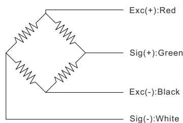
Torque channel(T)
